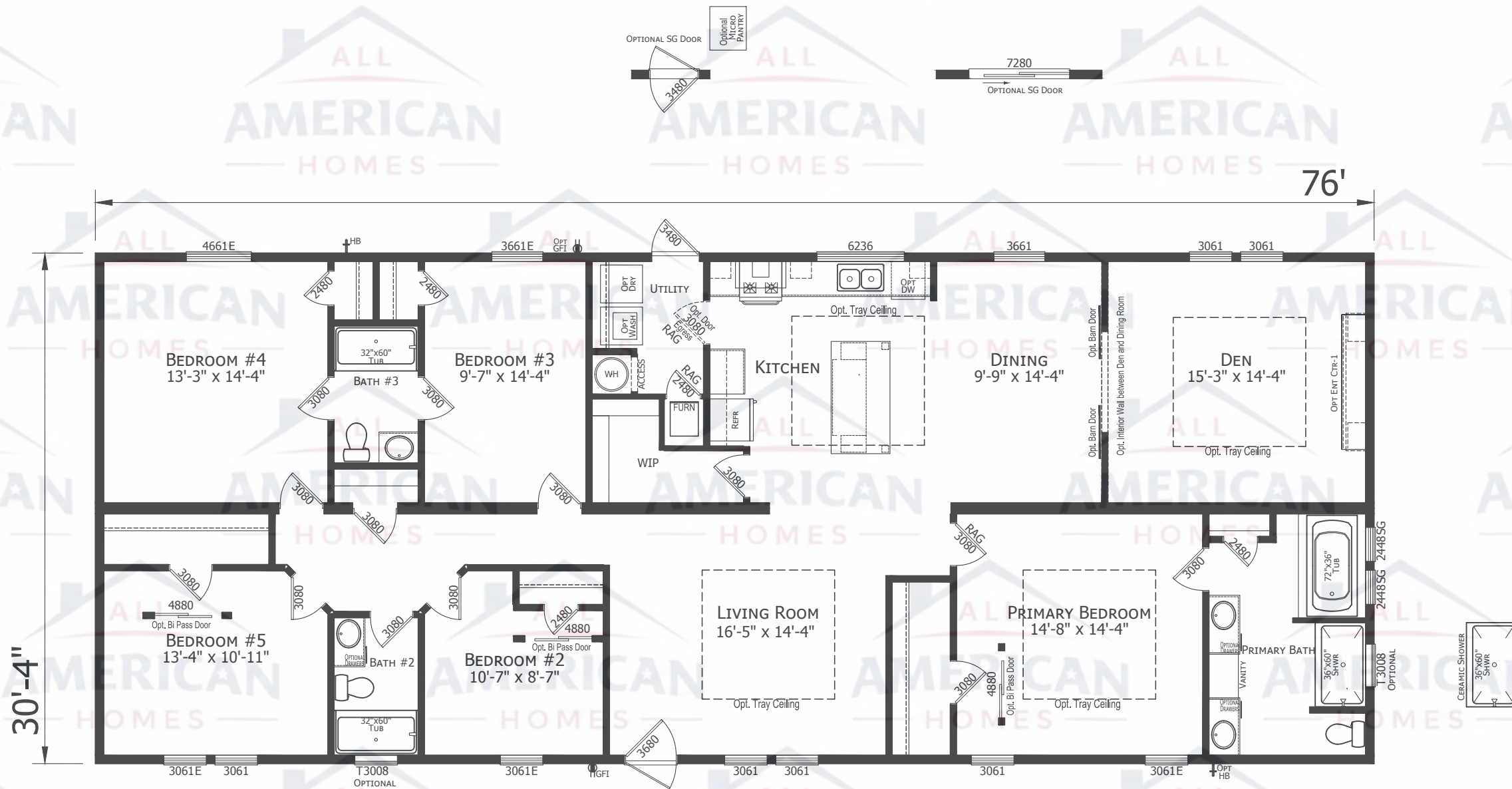
5 BEDROOM 3 BATH 76'-0" x 30'-4" 2305 Sq. Ft. TOTAL
