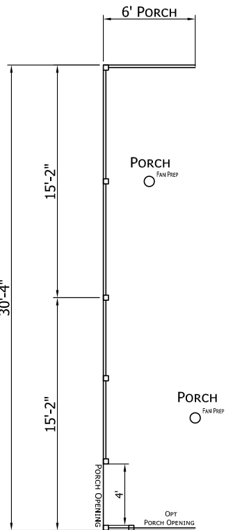
OPT 6' PORCH EXTENSION
